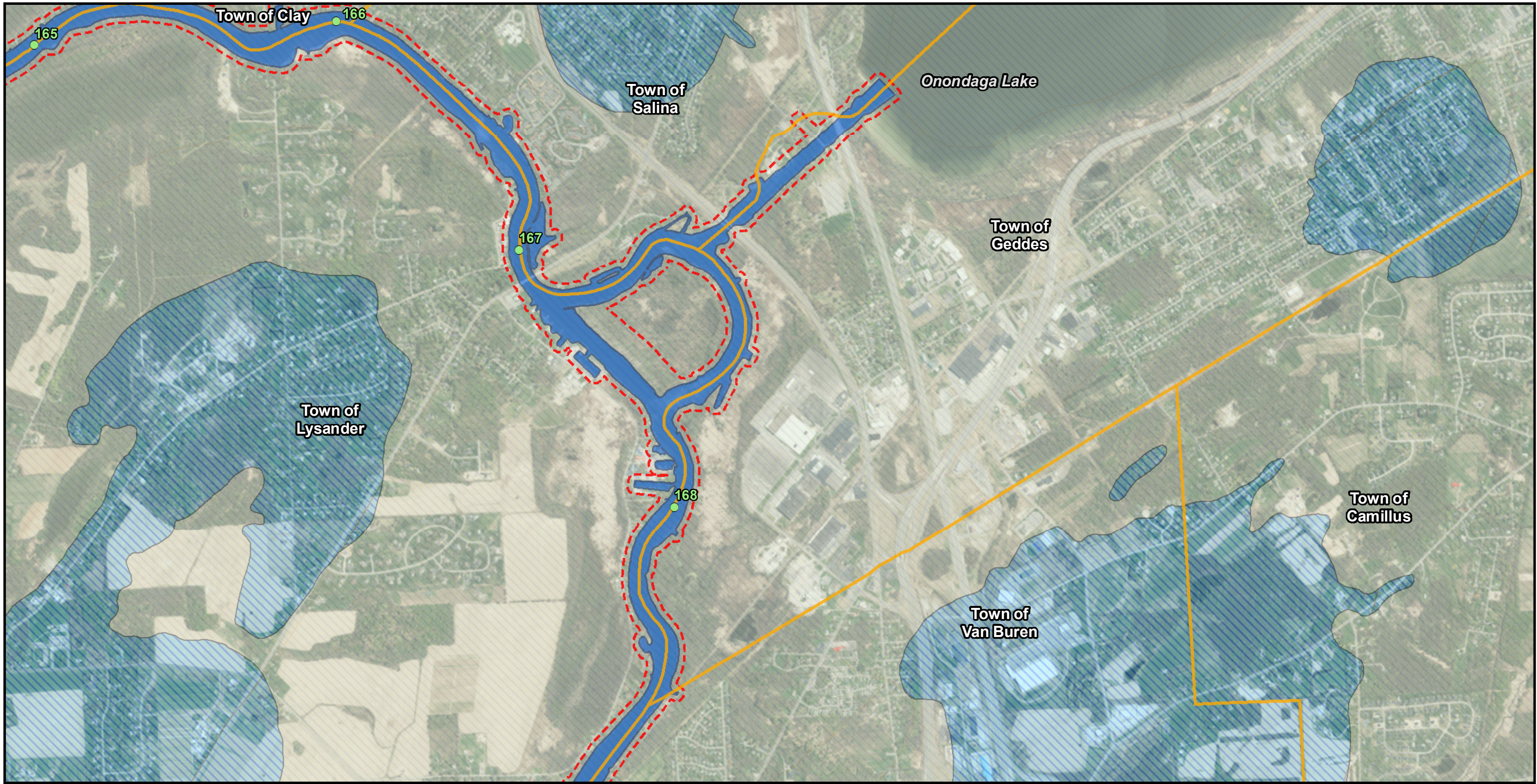
Figure 77F: Aquifers
